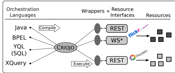
Fig. 2. The Pivot Architecture
