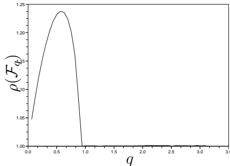
FIGURE 15. Spectral radius of the monodromy matrix modulo shifts \mathcal{F}_q .
