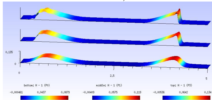
Figure 8 – Representation of H - 1 for t = 0.6 using P0 (bottom), P1 and P3 (top) polynomials.
