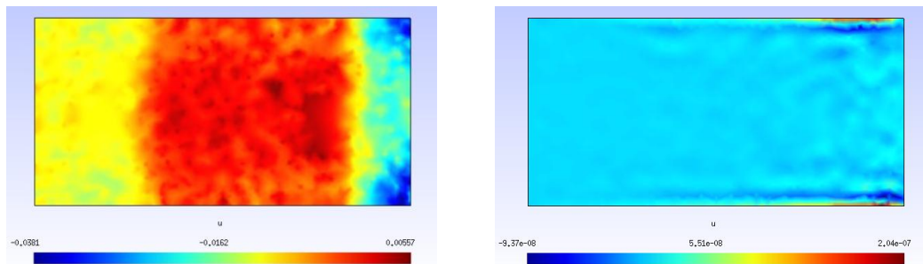
Figure 3b – Representation of u for P0 (left) and P3 (right) approximations at t = 0.1 .
