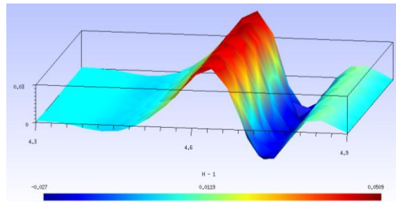
Figure 6 – Representation of H - 1 at t = 0.65 using a P1 approximation with no MOOD procedure.
