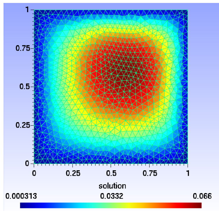
Figure 6 – Results for Patankar scheme with mesh M2.
