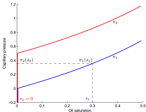
Figure 6: Capillary pressure connection at t = 0
