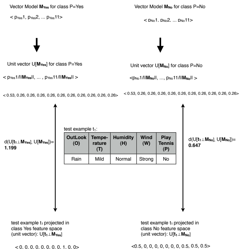
Figure 4: Test example on Play tennis data-set by LODE
