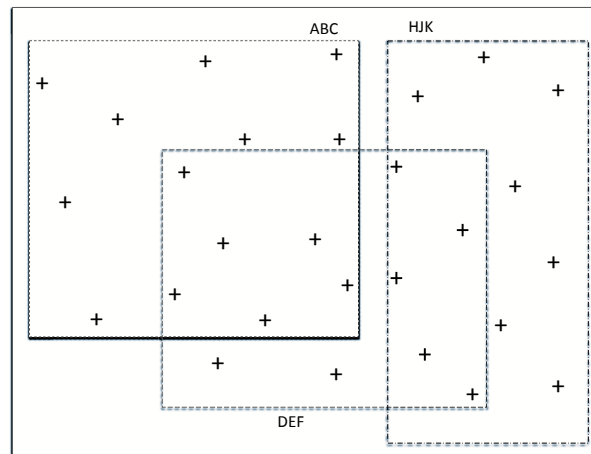
Figure 1: Difference between the induction of classification rules by covering and by possibly overlapping rules, like in LODE
