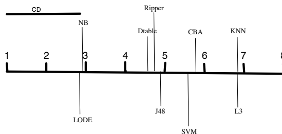
Figure 26: Graphical representation of Friedman test on results of Figure 25
