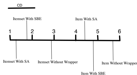
Figure 28: Graphical representation of Friedman test on results of Figure 27
