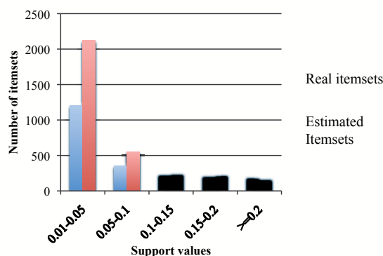
Figure 8: Histogram on the number of itemsets in class malignant of Breast .
