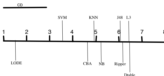
Figure 20: Graphical representation of Friedman test on results of Figure 19
