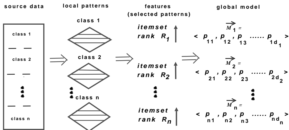
Figure 2: Work-flow of LODE according to the LEGO approach
