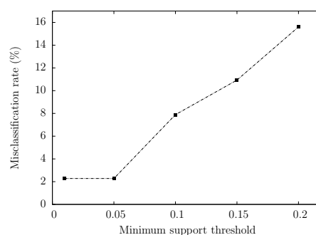
Figure 7: Misclassification on Wisconsin-Breast-cancer by class models on frequent itemsets at different minimum support
