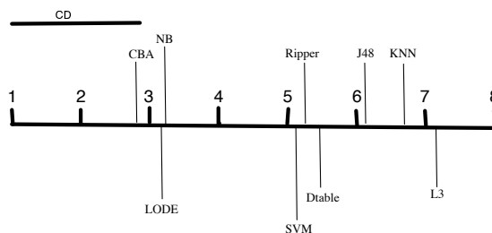
Figure 24: Graphical representation of Friedman test on the results of Figure 23
