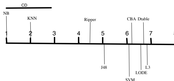
Figure 16: Graphical representation of Friedman test on differences between training times
