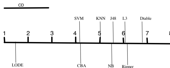
Figure 12: Graphical representation of Friedman test on differences in classification accuracy
