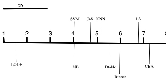
Figure 22: Graphical representation of Friedman test on results of Figure 21
