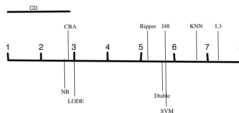
Figure 14: Graphical representation of Friedman test on results of Figure 13
