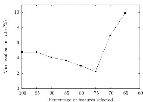
Figure 6: Error rate on Wisconsin-Breast-cancer with class models built on different number of itemsets
