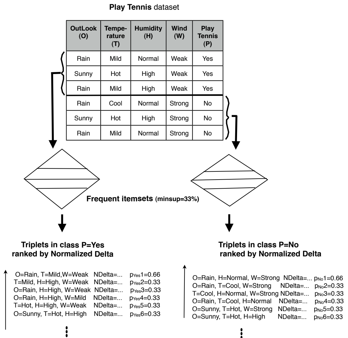
Figure 3: Example on Play tennis data-set by LODE
