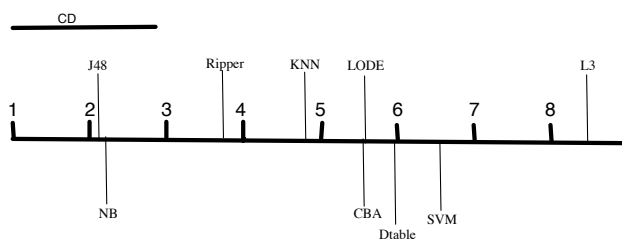
Figure 18: Graphical representation of Friedman test on differences between unit test times
