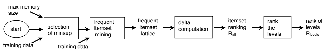
Figure 10: Initialisation of parameters and of tuning of LODE
