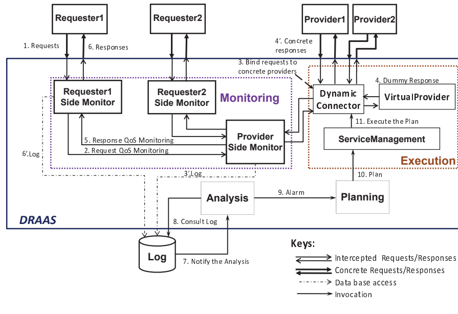
Fig. 2. DRAAS architecture
