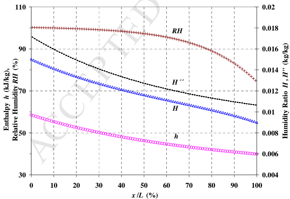
Fig. 14. Properties of the working air in the wet passage of the counter flow regenerative example.
