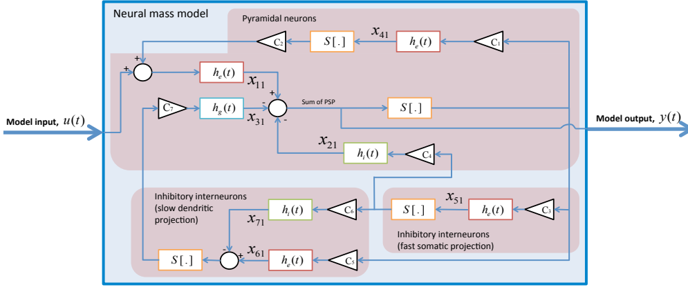
Figure 6. Detailed block diagram of the Wendling et. al. model. Reproduced from Figure 4 in [3].
