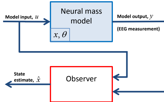
Figure 2. Block diagram of the neural mass model with our observer.
