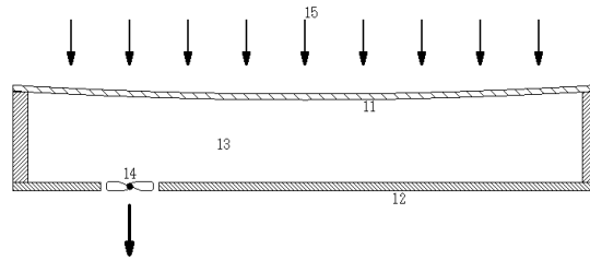
Figure 4: Transversal section of a mirror with its depression chamber
