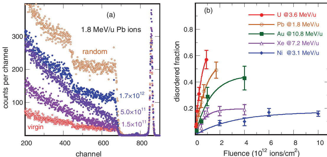
FIG. 11. (Color online) (a) C-RBS spectra of CaF 2 irradiated with 1.8-MeV/u Pb ions (full symbols) compared to virgin sample under channeling (along [111] axis) and random condition (open symbols). The fluence is given in units of ions per cm 2 . (b) Damage fraction deduced from C-RBS experiments as a function of fluence for different ion beams. Solid lines are exponential fits using a Poisson law [Eq. (5); Ref. 38].
