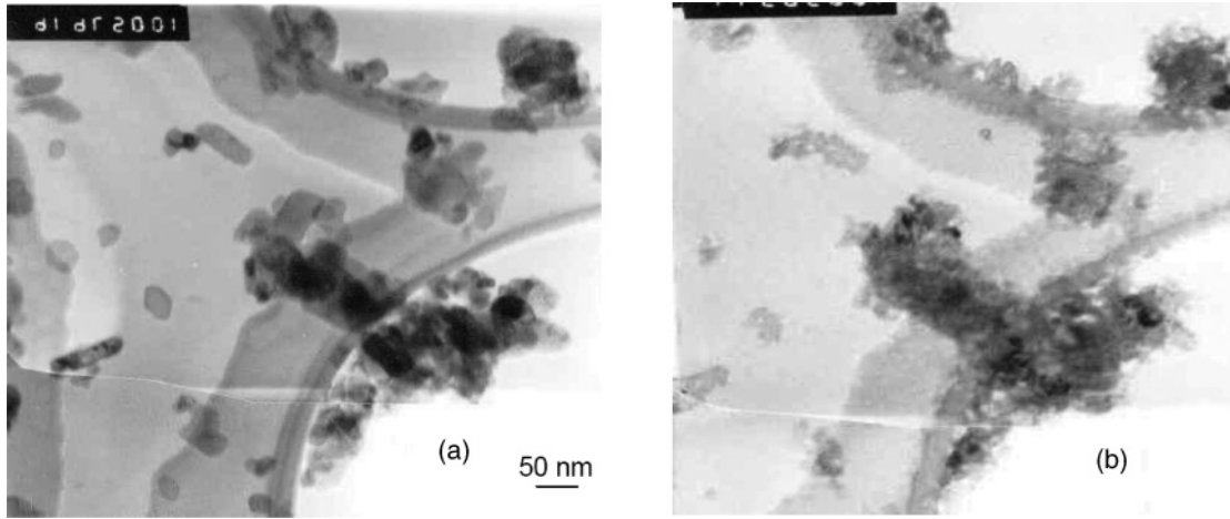
FIG. 10. TEM images of the same sample spot of CaF 2 powder taken (a) before and (b) after irradiation with 4.1-MeV/u Pb ions of fluence 10 12 ions/cm 2 .
