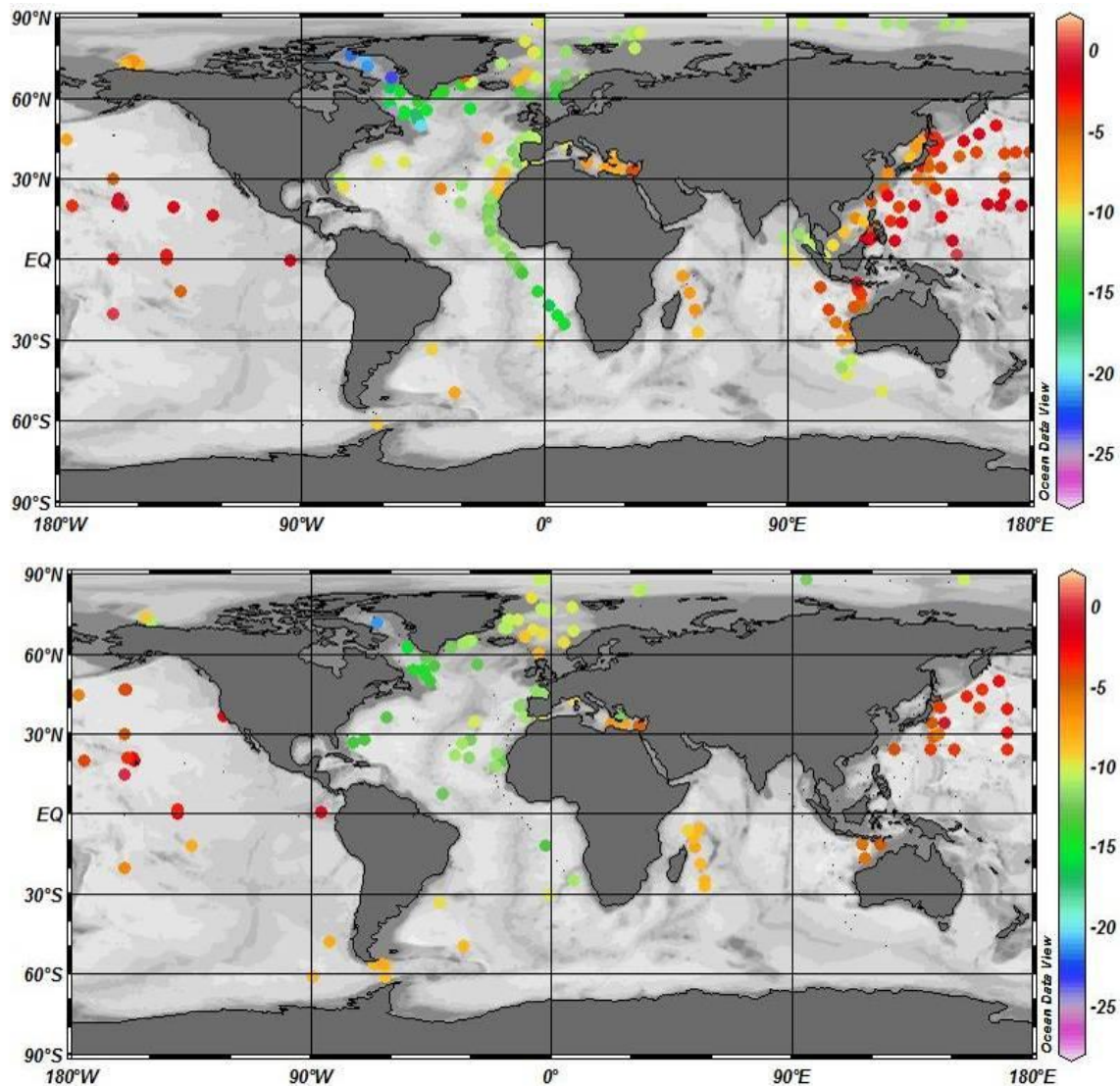
Fig. 4. \epsilon_{Nd} averaged between the surface and 400m depth (top) and between 800m depth and the bottom (bottom). Figure made with Ocean Data View [Schlitzer, 2009].
