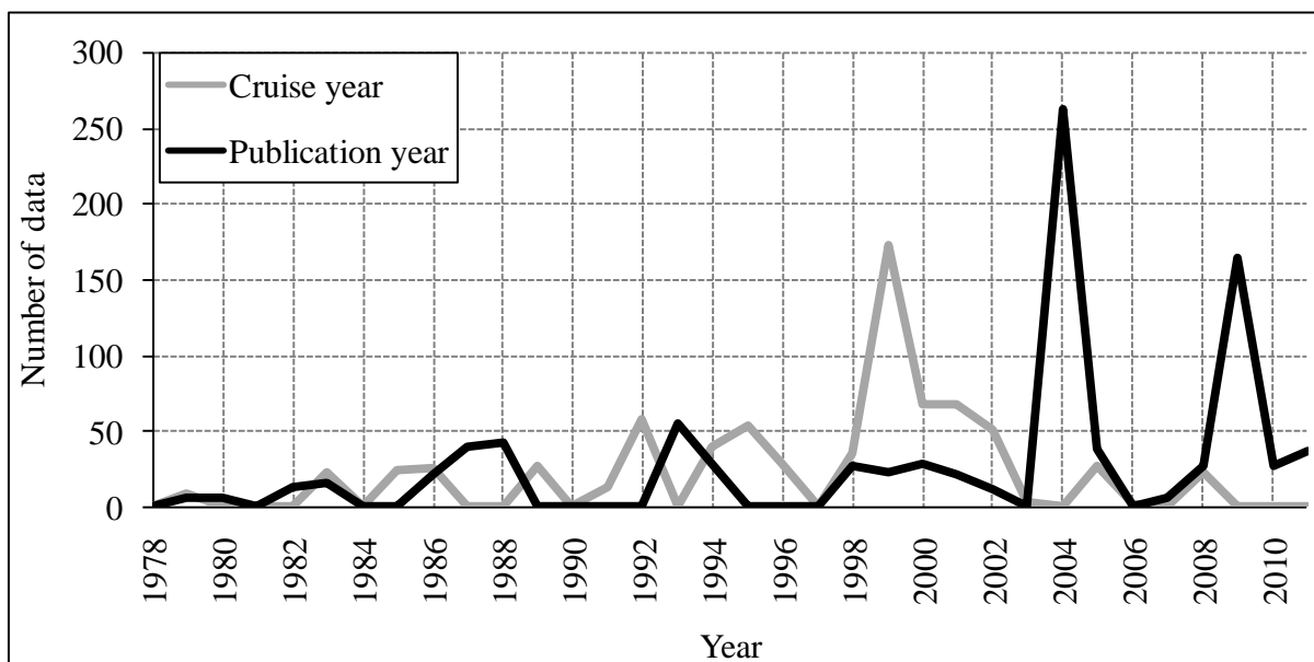
Fig. 6. Number of \epsilon_{Nd} data as a function of cruise and publication years. Note that cruise years are not always reported in the publications.
