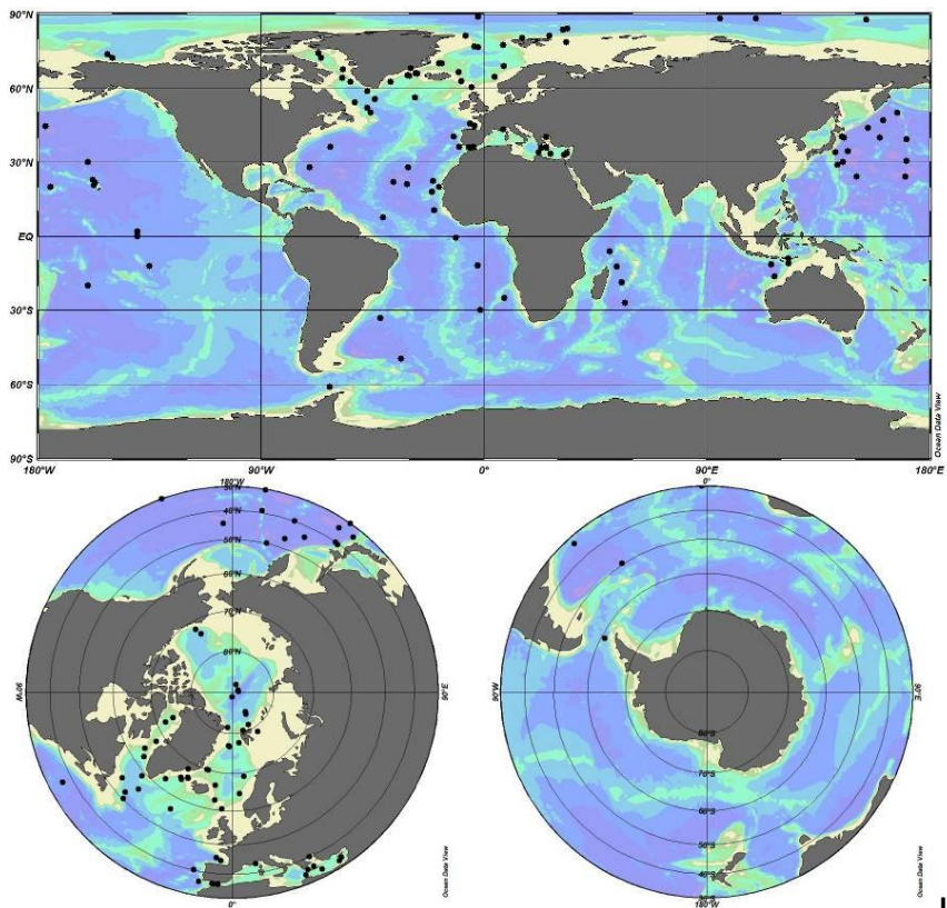
Fig 2. a: Location of all stations with \epsilon_{Nd} data. b: Location of stations with at least 3 \epsilon_{Nd} data per station. Figure made with Ocean Data View [Schlitzer, 2009].
