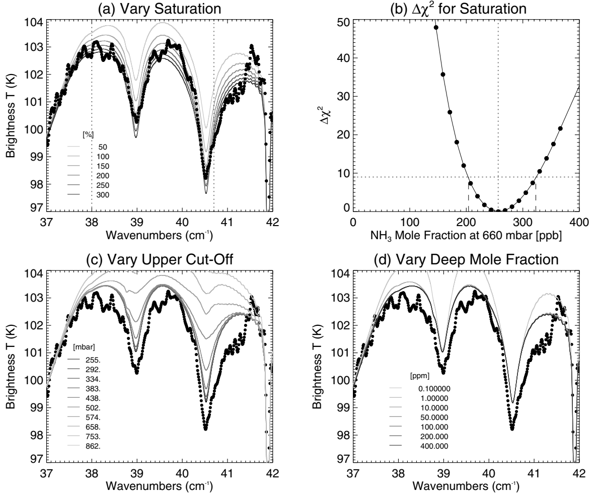
Fig. 8. Determining the most plausible fit for the \text{NH}_3 doublet. The vertical profile is parameterised in terms of a degree of saturation (panel a), with relative humidities given as percentages in the key, based on the best-fitting T(p) , an upper-level cut off (panel c), with pressures between 250–860 mbar given in the key) and a deep mole fraction (panel d), with mole fractions given in ppm in the key). Of the three parameters, the only way to increase the depth of the absorption features to match the SPIRE data (black circles) is to increase the relative humidity (panel a). The models in c) and d) do not match the data because they assume a relative humidity of 100%. The \Delta\chi^2 for each value of the relative humidity is evaluated for data between the two dotted vertical lines in panel a (i.e., avoiding artefacts in the data near 41.5 \text{ cm}^{-1} ) and displayed in panel b). The best-fit mole fraction at 660 mbar plus the 3\sigma uncertainty is shown in panel b).
