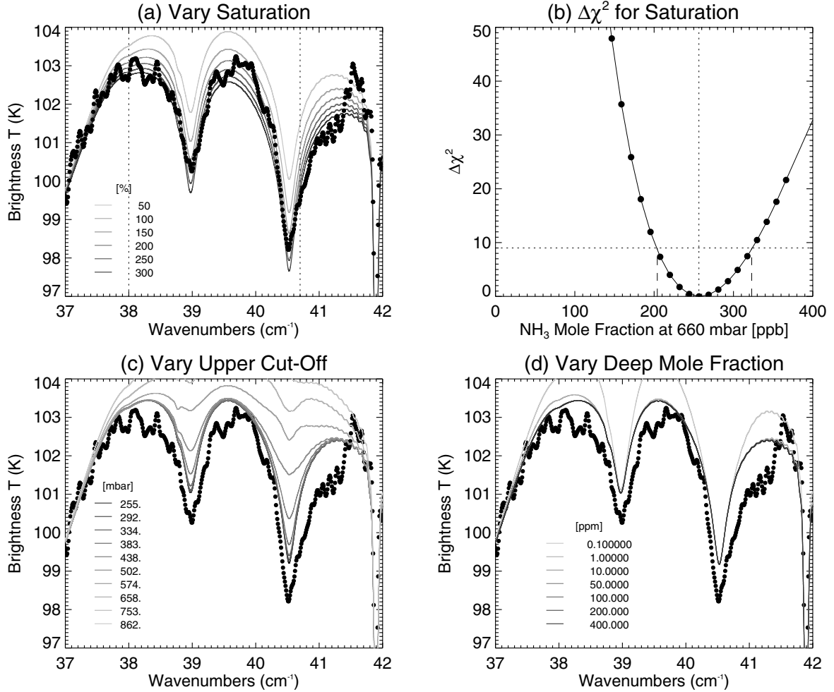
Fig. 8. Determining the most plausible fit for the NH 3 doublet. The vertical profile is parameterised in terms of a degree of saturation (panel a ), with relative humidities given as percentages in the key, based on the best-fitting T(p) , an upper-level cut off (panel c ), with pressures between 250–860 mbar given in the key) and a deep mole fraction (panel d ), with mole fractions given in ppm in the key). Of the three parameters, the only way to increase the depth of the absorption features to match the SPIRE data (black circles) is to increase the relative humidity (panel a ). The models in c and d do not match the data because they assume a relative humidity of 100%. The \Delta\chi^2 for each value of the relative humidity is evaluated for data between the two dotted vertical lines in panel a (i.e., avoiding artefacts in the data near 41.5 cm -1 ) and displayed in panel b ). The best-fit mole fraction at 660 mbar plus the 3\sigma uncertainty is shown in panel b .
