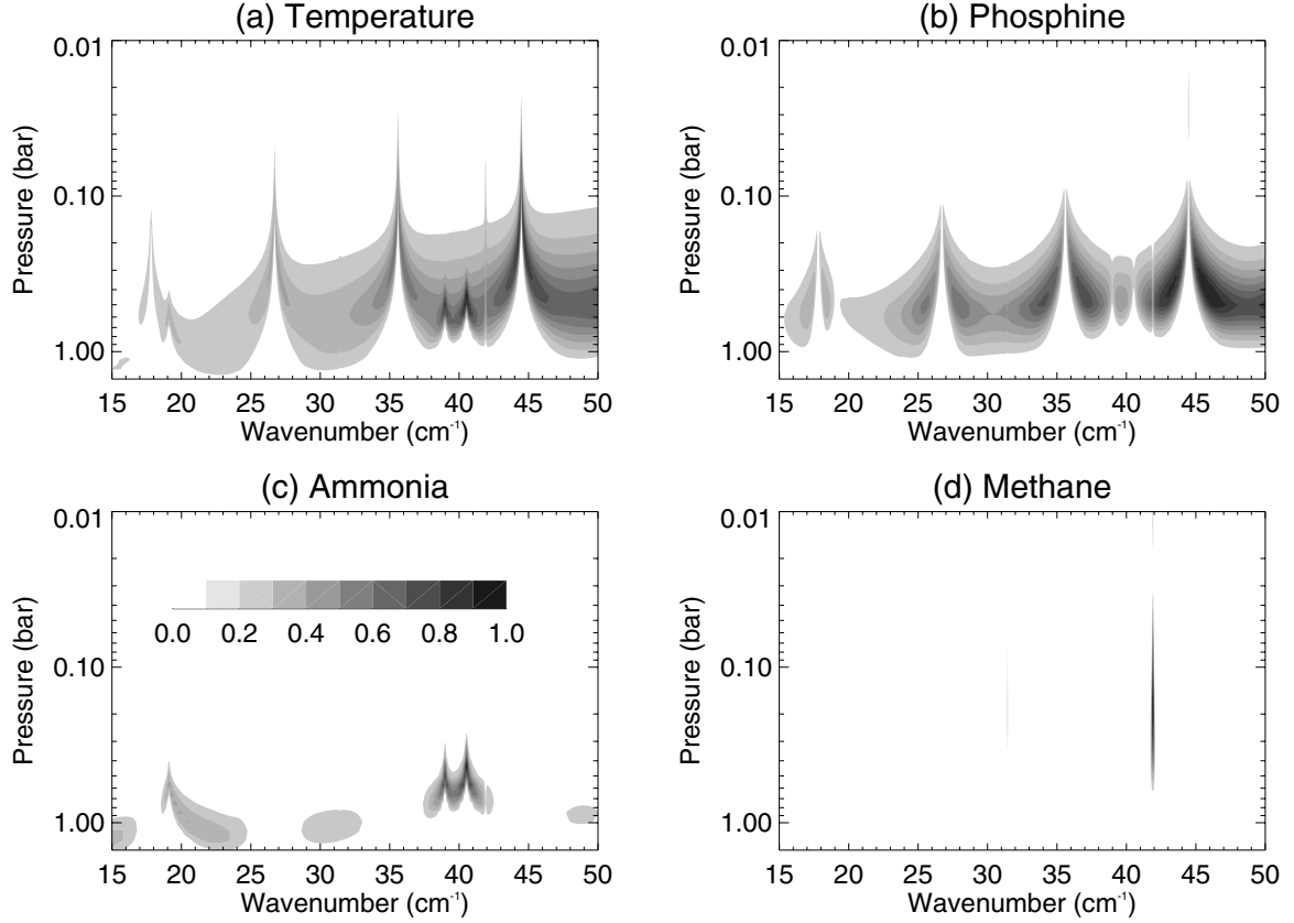
Fig. 4. Functional derivatives (rate of change of radiance with respect to the model parameter) for the four major contributors to the sub-millimetre spectrum. Figures have been normalised, and each contour represents a change of 0.1. A scale bar is provided in panel c).
