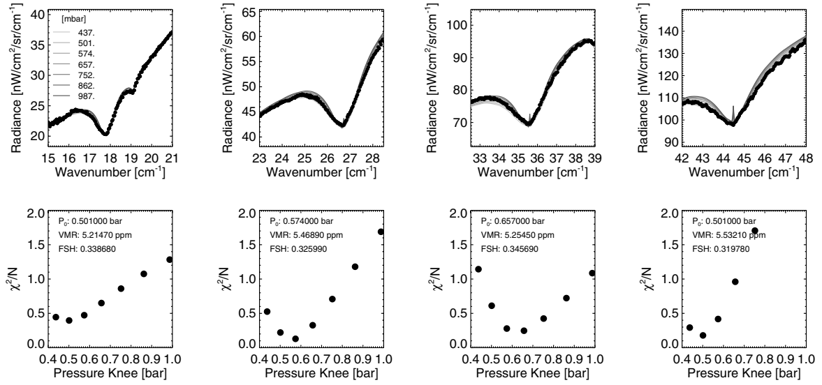
Fig. 6. Testing the sensitivity to the pressure knee of the PH 3 vertical distribution. The pressure levels (in mbar) are given by the key in the top left corner , but the differences between these curves is hard to distinguish in the top four panels , showing the difficulty we face in trying to constrain the pressure knee from these data. The \chi^2/N distributions in the bottom panels show convergence on the 500–650 mbar range. The \chi^2 estimates do not include the spurious emission peaks from the models (see main text and Fig. 7). The best fitting pressure knee, deep mole fraction and fractional scale height are provided in the lower panels .
