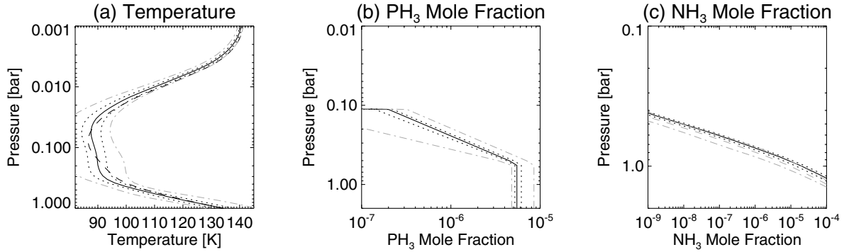
Fig. 5. Retrieved vertical profiles for temperature, PH 3 and NH 3 in the best-fitting case. The solid line shows the retrieved profile, the dotted line is the uncertainty on the retrieval, estimated by applying a 5% shift in the measured radiances (the absolute calibration uncertainty) and redoing the calculation. The dashed line in the temperature plot a ) is a global mean of the T(p) profiles retrieved from the Cassini /CIRS far-infrared focal plane between 2004 and 2008. The dot-dashed grey lines in a ) and b ) are temperature and PH 3 retrievals based on extreme estimates of the calibration uncertainty of \pm 15\% . The NH 3 profile in c ) was estimated by scaling the saturated vapour pressure profile (see Fig. 8), so the uncertainties are the same at all altitudes. The grey dashed line in c ) is the saturated vapour pressure curve of NH 3 assuming a relative humidity of 100%, the dot-dashed grey line use the temperature profiles given by the dotted lines in a ). The uncertainty in the saturated mole fraction is greater than the uncertainty on the retrieved abundances of NH 3 .
