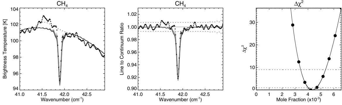
Fig. 9. Testing the line-by-line forward model by fitting the CH 4 rotational line. The left hand panel shows the brightness temperatures, with the data given by circles, the smooth spline-fit to the continuum as the dotted line, and the solid grey lines showing the range of mole fractions tested. The central panel converts this to a line-to-continuum ratio relative to the smooth spline. Here, the dotted lines show the error envelope as defined in the main text. The right hand panel shows the \Delta\chi^2 for the model, with dotted horizontal lines showing the 1\sigma and 3\sigma confidence limits on the results. The derived methane abundance depends upon the choice of line data, with a mole fraction of (4.3 \pm 0.3) \times 10^{-3} assuming line intensities from Wishnow et al. (2007) (shown here) and (4.8 \pm 0.3) \times 10^{-3} using intensities from Boudon et al. (2010) .
