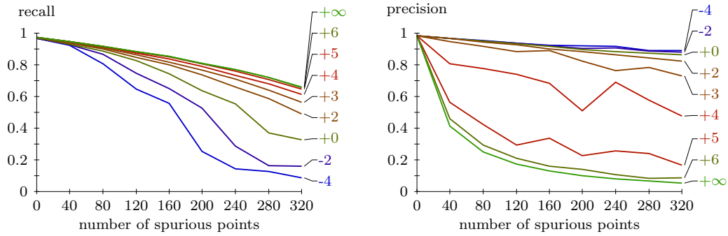
Fig. 17 Influence of the NFA threshold ( \epsilon ). We consider the same experiment as in Fig. 10 (that is, 20 real trajectories spanning 20 frames, with a given number of spurious points in each frame), and examine the influence of the threshold \epsilon arising in the NFA algorithm. Recall and precision curves are plotted in function of the number of spurious points, for different values of \log_{10} \epsilon (ranging from -4 to +\infty ). We can see that the good precision control predicted by the theory for \epsilon \leq 1 ( \log_{10} \epsilon \leq 0 ) is well achieved, since the first significant precision losses occur around \log_{10} \epsilon = 3 . Hence, the default value \log_{10} \epsilon = 0 is a good compromise in this experiment, even if slightly better recalls (without significant precision losses) can be achieved by using greater values like \log_{10} \epsilon = 2 .
