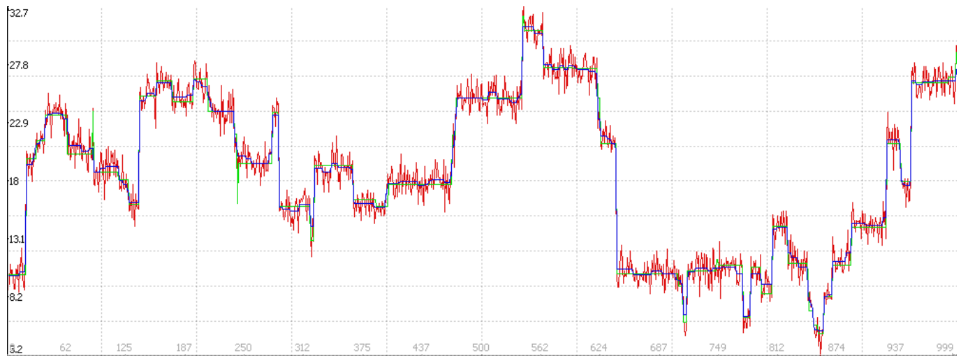
Fig. 3. In this example, y (in red) is a piecewise constant process of size N = 1000 (unknown ground truth, in green) corrupted by additive Gaussian noise of unit variance. The TV-denosed signal x^* , with \lambda = 2 , is in blue.
