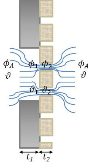
FIG. 3. (color online)Viscous flow of the fluid through the perforations. Downstream the perforation, the “apparent” fluid velocity in the mesh is increased because of the squeezing due to the presence of the perforations upstream. This results in an “effective flow resistivity” that accounts for this diaphragm effect.
