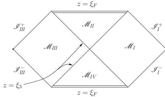
Figure 3.1. \hat{\mathcal{M}} with its various subsets. For example, \mathcal{M}_{I \cup II} is the union of \mathcal{M}_I and of \mathcal{M}_{II} and of that part of \{z = \xi_3\} which lies in the intersection of their closures; this is the manifold constructed in [13]. Very roughly speaking, the various \mathcal{S} 's correspond to x = z = \xi_1 . It should be stressed that this is neither a conformal diagram, nor is the space-time a product of the figure times S^2 \times S^1 : \mathcal{M}_I cannot be the product of the depicted diamond with S^2 \times S^1 , as this product is not simply connected, while \mathcal{M}_I is. But the diagram represents accurately the causal relations between the various \mathcal{M}_N 's, as well as the geometry near the bifurcate horizon z = \xi_F , as the manifold does have a product structure there.
