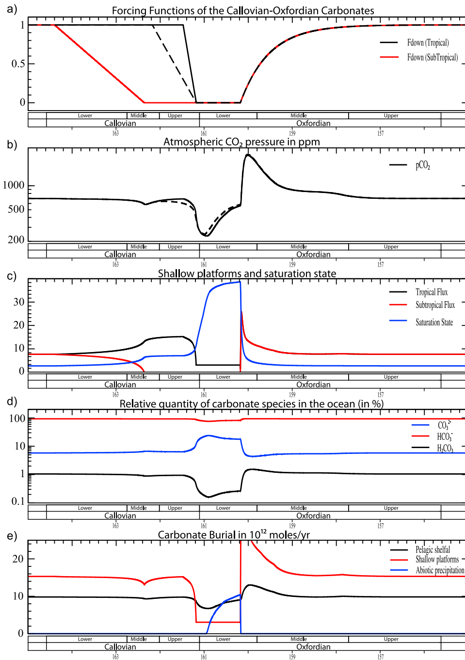
Figure 1. Model results simulating the effects of the collapse and the recovery of the carbonate platforms during the Middle Late Jurassic transition. (a) F_{down} function as described in the main text. (b) Changes in atmospheric CO_2 content. Note that the first collapse is more diluted in times than the second one based on geological data. Nevertheless, the effect remains the same when increasing the time for the collapse (see dashed curve). (c) Changes in the burial flux coming from tropical and subtropical platforms. Note the remaining flux of the tropical shallow carbonate platform during the crisis (i.e., 20% here). We have also plotted the mean saturation state. (d) Distribution of the carbonate species. (e) Changes in sedimentary calcium carbonate burial fluxes. The black curve represents the neritic platform carbonate burial flux, the red curve represents the pelagic shelfal carbonate burial, and the green curve represents “abiotic” carbonate production flux (see text). Note that the neritic/global carbonate production ratio is 65% in this run. Platform collapse lasts for 1 million years; 20% of the preperturbation platform burial flux is conserved during the crisis in order to account for the likely possibility that carbonate platforms still exist in specific environments.
