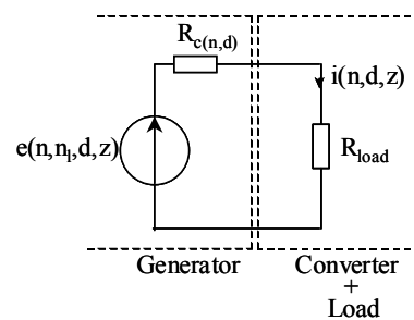
Fig. 20: Electrical diagram
