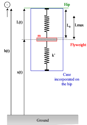
Fig. 4: Mechanical structure of a linear generator
