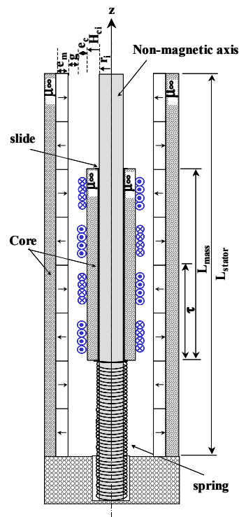
Fig. 14: Simplified generator diagram (longitudinal section cut)
