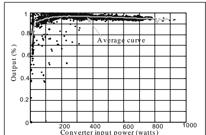
Fig. 9: Cloud of points for converter output and the corresponding average curve
