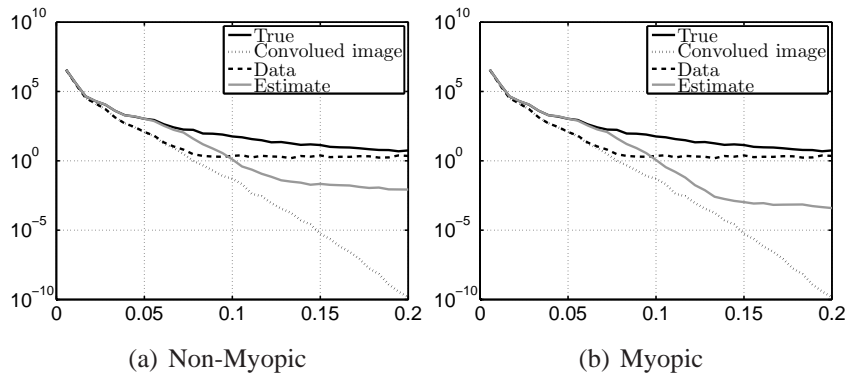
Fig. 3. Circular average of the empirical power spectral density of the image, the convolved image, the data (convolved image corrupted by noise) and the estimates, in radial frequency with y-axis in logarithmic scale. The x-axis is the radial frequency.
