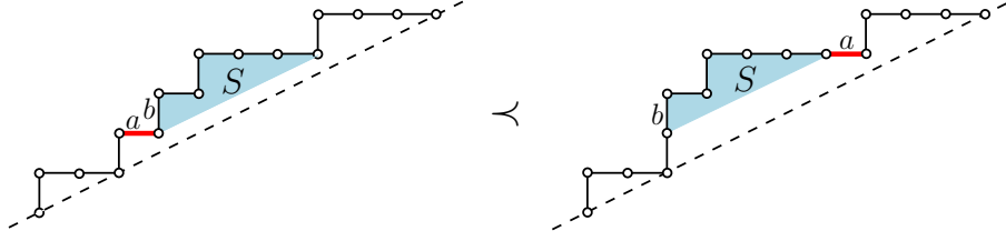
FIGURE 1. The covering relation between m -ballot paths ( m = 2 ).
