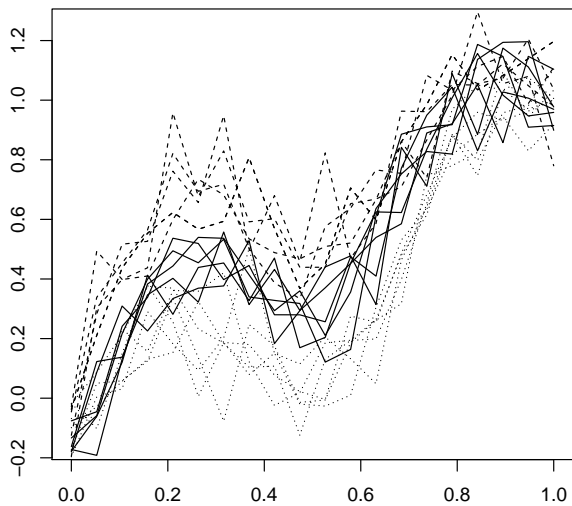
Figure 5. Example of functions. Functions based on \sqrt{x} are on dashed lines, ones based on x are on solid lines and ones based on x^2 are on dotted lines.
