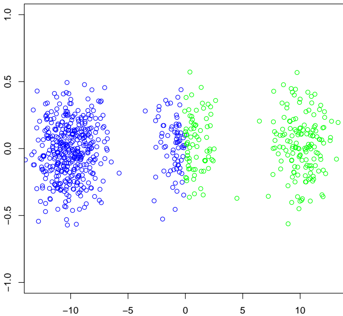
Figure 1. First iteration of X-Alter algorithm (Step 1.)
