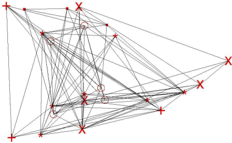
Figure 1: Example of a simulated graph: the vertices of the 5 cliques are represented by different labels (+ \square * x o)
