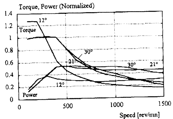
Figure 9: Influence of \beta_r on torque and power characteristics (control in trapezoidal torque waveform)
