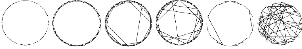
Figure 3: Typical emergent networks obtained with \delta = 0.15, \delta = 0.3, \delta = 0.35, \delta = 0.7, \delta = 0.98 . The last network has been generated with the standard connections model of Jackson and Wolinsky with \delta = 0.7 and a connection cost equal to 0.5 (A (fixed) link cost in the standard connections model set to 0.5 is approximately equal to the average (potential) link cost borne in the spatialized connections model with 20 agents).
