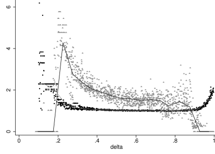
Figure 2: Average distance (black circles: d(g)/d(g^{rd}) ), average clustering (grey triangles: c(g)/c(g^{rd}) ) and their fitted values of emergent networks for 1,500 simulations with randomly drawn values of \delta \in ]0, 1[ .
