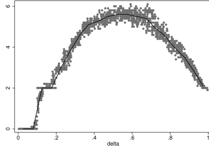
Figure 1: Average degree \hat{\eta}(g) of emergent networks for 1,500 simulations with randomly drawn values of \delta \in ]0; 1[ .
