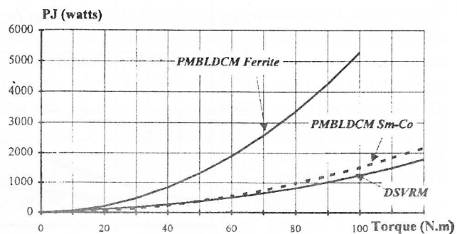
Fig. 10. Copper losses vs. average torque for DSVRM and PMBLDCM.
