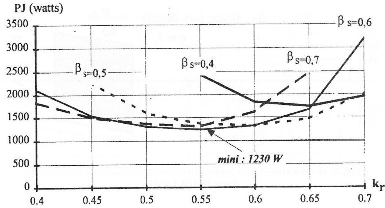
Fig. 5. Influence of airgap radius to outer radius ratio on the copper losses for a 6/4 three-phase DSRVM ( T = 100 Nm, R = 125 mm, L = 150 mm, k_b = 60\% ).
