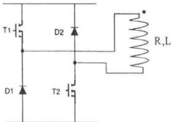
figure 2: example of power converter with an asymmetric half bridge per phase.
