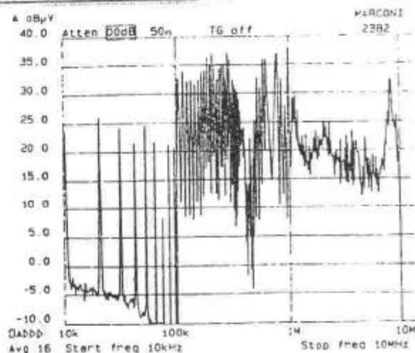
figure 26 : PWM conducted perturbations in common mode measurements.
