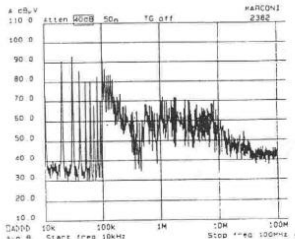
figure 24 : PWM conducted perturbations in differential mode measurements.
