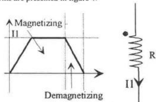
figure 4: current modelling. Machine fed by a full wave voltage.
