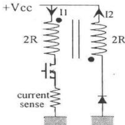
figure 3: example of bifilar machine with it's power converter.
