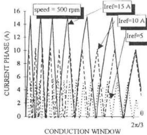
figure 11 : computing simulation of current wave-forms in SELF SWITCHING mode with speed=500rpm; different current references from 5A to 15A.
