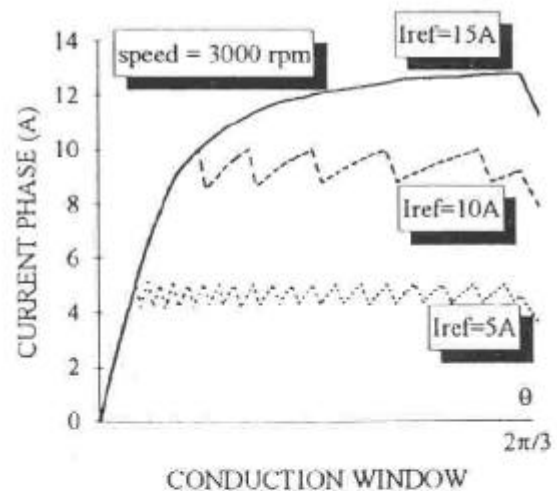
figure 12 : computing simulation of current wave-forms in PWM mode with T_{off}=cst and speed=3000rpm; different current references from 5A to 15A.
