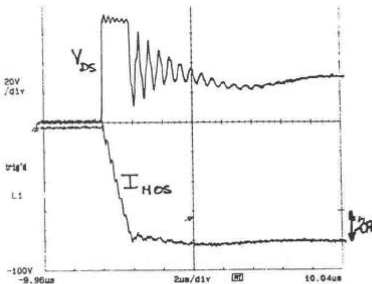
figure 18: real commutation wave-forms commutation for the MOS; Average current=5A
