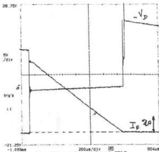
Figure 17: real commutation wave-forms in SELF SWITCHING mode with standard diodes(1N5408); Average current=5A.
