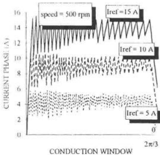
figure 10 : computing simulation of current wave-forms in PWM mode with T_{off}=cst=10\mu\text{s} and speed=500rpm; different current references from 5A to 15A.
