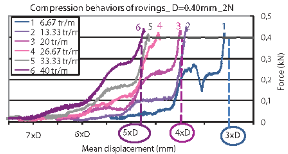
Figure 9. The twist effect on compression behaviors of rovings with a filament diameter of 0.40 mm and a tension of 2 N.
