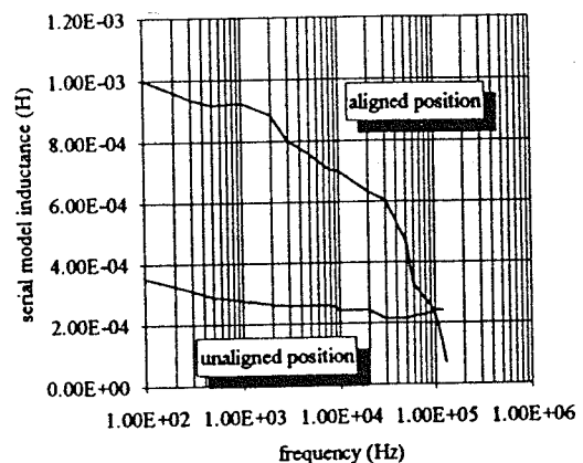
figure 3 : influence of frequency upon the serial inductive parameter :condition 20mA rms.
