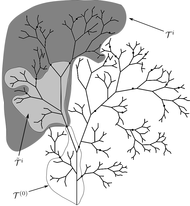
FIGURE 2. The tree \mathcal{T}_0 , \mathcal{T}^{(0)} , and a tree \mathcal{T}^i and its sub-tree \tilde{\mathcal{T}}^i belonging to the first generation tree \mathcal{T}^{(1)} \setminus \mathcal{T}^{(0)} .
