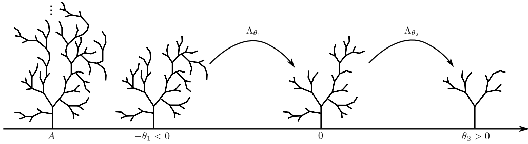
FIGURE 1. The pruning process, starting from explosion time A defined in (32).
