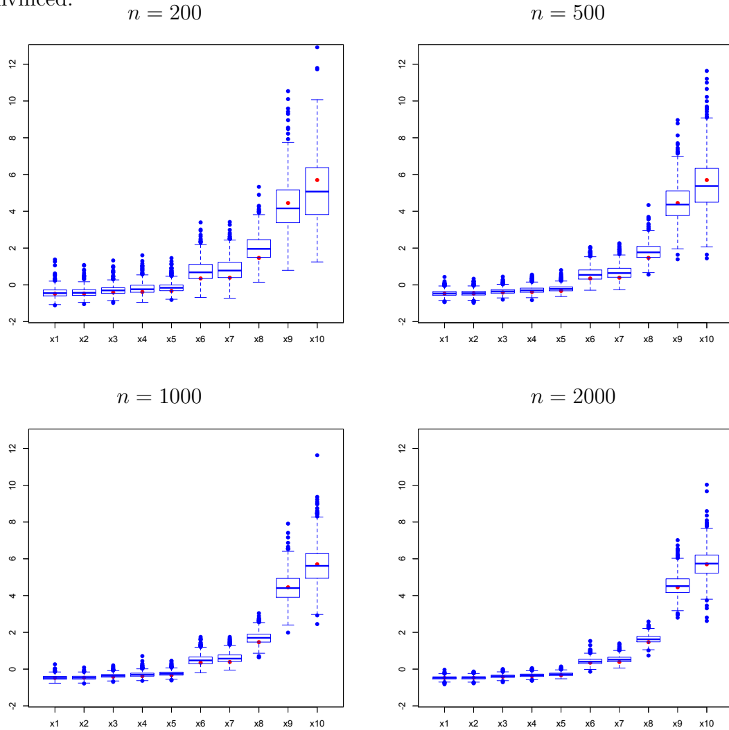
Figure 4.2. Almost sure convergence of \widehat{f}_n(\widehat{\theta}'_n x) to f(\theta'x) for 10 different values of x .
