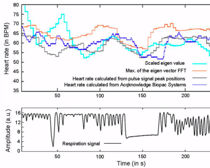
Figure 8. Heart rate estimation calculated with 3 methods thanks to SSA, heart rate reference given by Acqknowledge Biopac software (top); Respiration signal with simulated apnea (bottom).
