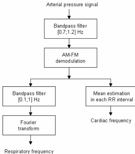
Figure 2. AM-FM demodulation diagram
