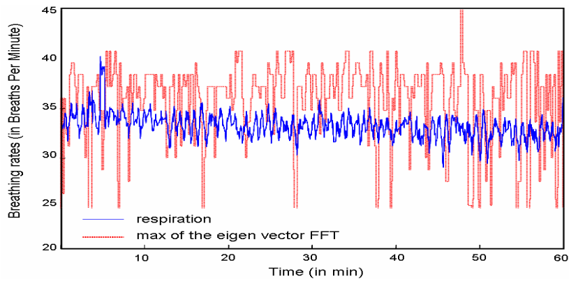
Figure 12. Breathing rate obtained from respiration signal (peaks counting) and with maximum value of the FFT of the reconstructed signal
