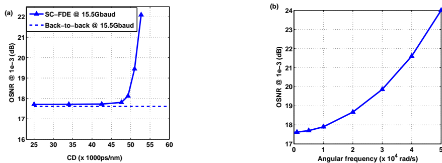
Fig. 2. (a) OSNR performance at \text{BER} = 10^{-3} vs. CD (DGD = 90ps) ; (b) Dynamical behavior of the adaptive SC-FDE
