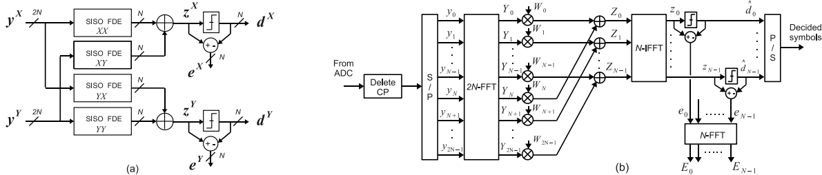
Fig. 1. The SC-FDE architecture: (a) The joint CD and PMD equalizer, (b) The SISO FDE
