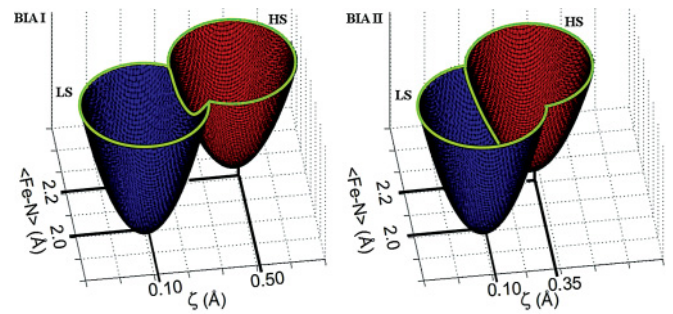
FIG. 10. (Color online) Two-mode description of on-site molecular potentials for BIA I and BIA II as a function of the average \langle \text{Fe} - \text{N} \rangle bond length ( \text{\AA} ) and of the length distortion parameter \zeta = \sum_{i=1}^6 |\text{Fe} - \text{N}_i - \langle \text{Fe} - \text{N} \rangle| ( \text{\AA} ).
