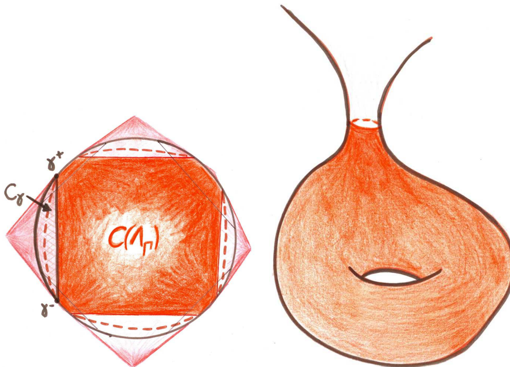
FIGURE 2. Convexe-cocompact
