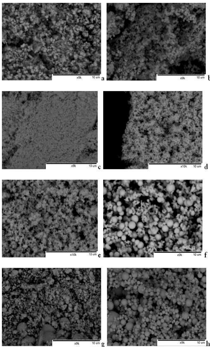
51 Fig. 3 SEM images of nanobeads obtained by forced hydrolysis: a – NBI*, b – NBII**, c – 52 NBIII*, d – NBIII**, e – NBIV*, f – NBIV**, g – NBVI*, h – NBVI** 53 54 55 56 57
