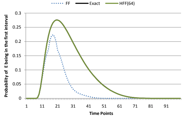
Figure 2: M^t(E \in [0, 1])
