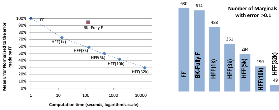
Figure 6: (a) Normalized mean errors over all marginals, (b) Number of marginals with error greater than 0.1: NGF-stimulation
