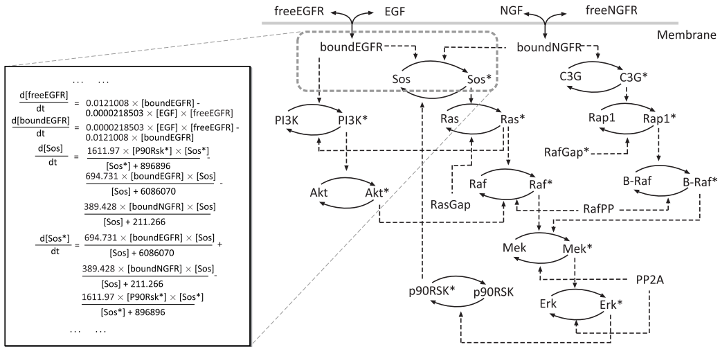
Figure 3: EGF-NGF pathway
