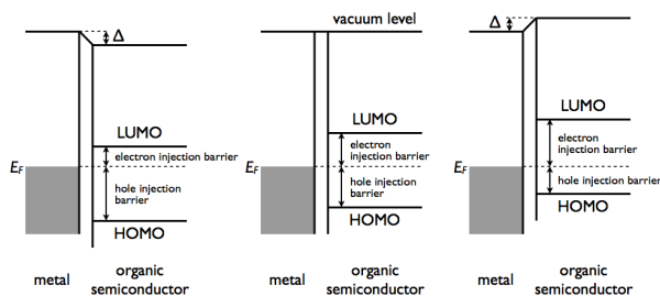
Figure 5. Energy diagram of the metal-organic semiconductor interface. Center: no interface dipole (vacuum level alignment). Left and right: Upon formation of an interface dipole \Delta , the energy levels shift, thus inducing a change of the injection barriers. HOMO and LUMO stand for Highest Occupied Molecular Orbital and Lowest Unoccupied Molecular Orbital; E_F is the metal Fermi level.
