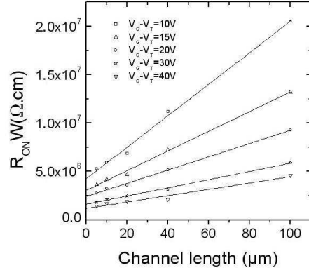
Figure 4. Illustration of the Transfer Line Method for various gate voltages.
