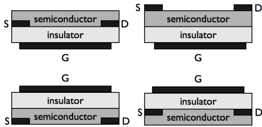
Figure 2. Diagram of the thin-film transistor (TFT) architecture. S: source; D: drain; G: gate; Top down and from left to right: bottom gate, bottom contact; bottom gate, top contacts; top gate, bottom contacts; top gate, top contacts.
