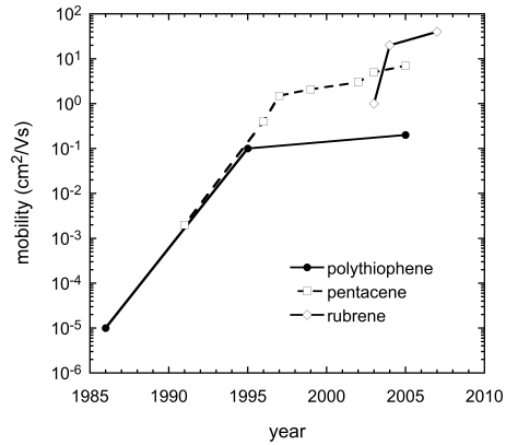
Figure 3. Improvement of the mobility for three organic semiconductors used in organic transistors, one polymer (polythiophene) and two small molecules (pentacene and rubrene). Data on rubrene pertains to single crystals.
