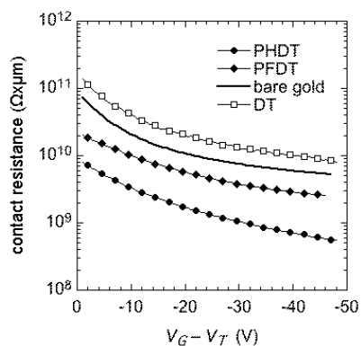
Figure 6. Gate voltage dependent contact resistance as measured by TLM on bottom gate, bottom contact organic transistors with pentacene semiconductor and gold source and drain electrodes. The gold electrodes were modified with various thiol-based SAMs bearing various dipole moments.
