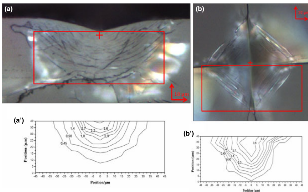
Fig. 6. Optical microscope and Raman mapping of the iso-density curves for a 20 N Vickers load in side view (a,a') and top view (b,b').
