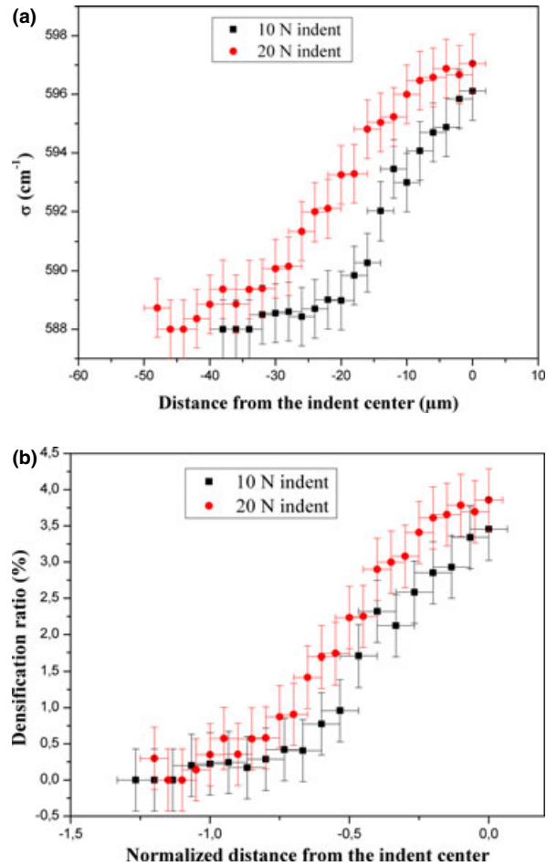
Fig. 4. (a) Top view mapping of the Raman shift of the centroid of the band outside a precrack domain for 10 N and 20 N Vickers loads. (b) Top view mapping of the densification ratio as function as the normalized distance from the indent center outside a precrack domain for 10 N and 20 N Vickers loads.
