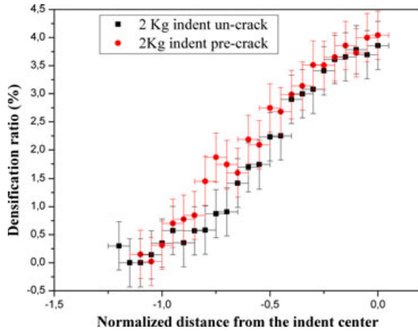
Fig. 5. Top view mapping of the densification ratio as function of the normalized distance from the indent center for 20 N indent outside (black square) or on a precrack line (red circles).
