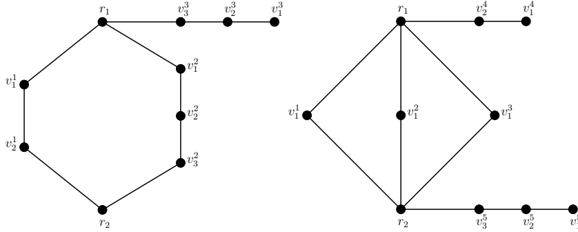
Figure 2: The partial balloons PB(2, 3, \overline{3}) and PB(1, 1, 1, \overline{2}, 3)
