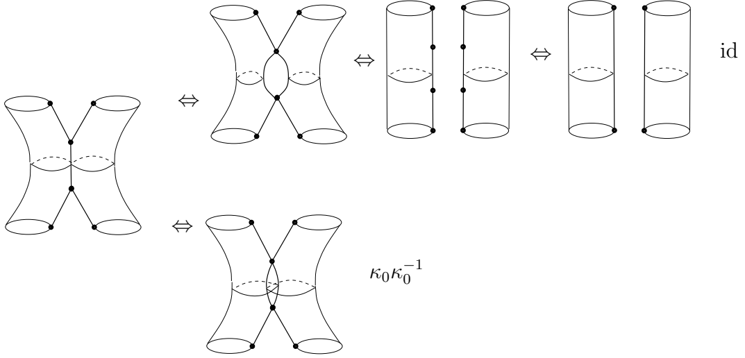
Figure 14: The spin foams \text{id} and \kappa_0 \kappa_0^{-1} can be consistently deformed into each other by application of the pulling moves described above (and their inverses), and removing/adding trivial vertices.
