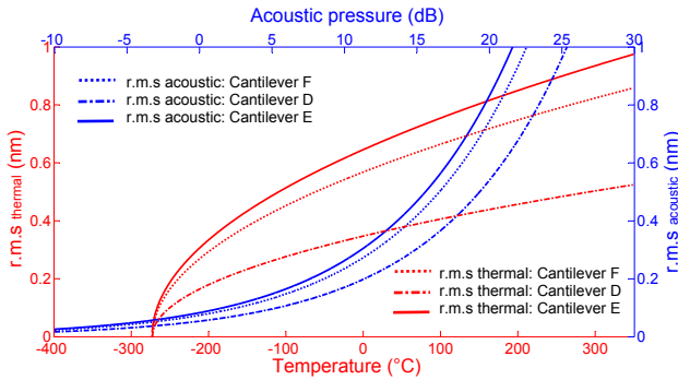
FIG. 10. Enlarged view of noise interferences in the cantilevers E, D and F.
