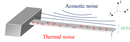
FIG. 1. Simplified scheme of an AFM cantilever subject to thermal and acoustic noises.
