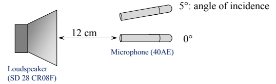
FIG. 14. Simplified scheme showing the position of the microphone according to two different angles of incidence.
