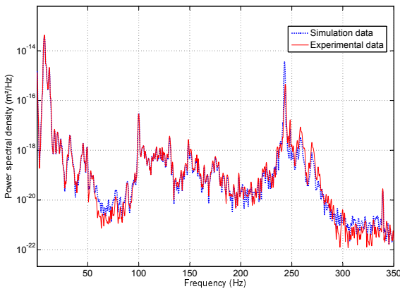
Fig. 23. Power spectral density of the cantilever 2 tip vibrations subject to ground motion (condition 1).
