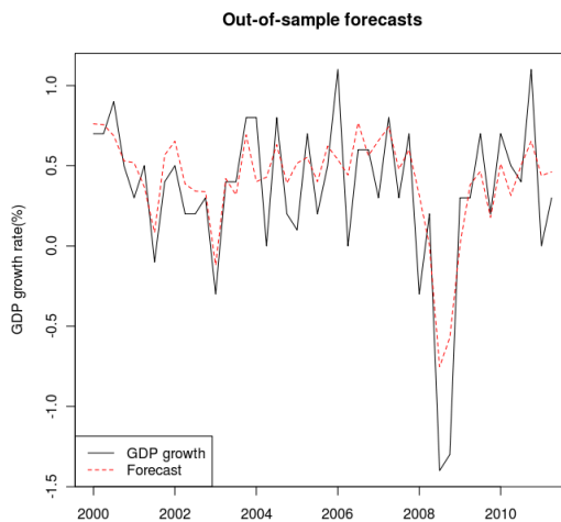
Figure 1: French GDP online prediction using the quantile loss function with \tau = 0.5 .
