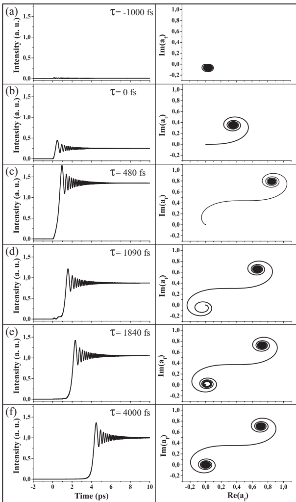
FIG. 4. Left: Temporal evolution of the final population during the probe pulse (normalized to the population at long time and delay); Right: Corresponding probability amplitude plotted in the complex plane. Pump-probe delays are -1000 fs (a), 0 fs (b), 480 fs (c), 1090 fs (d), 1840 fs (e), 4000 fs (f)
