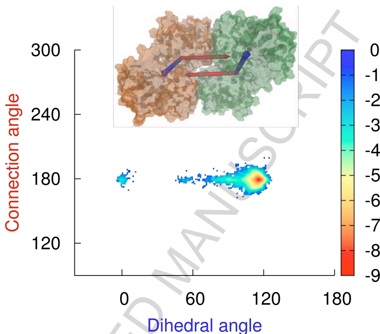
Figure 2: Angular free energy (kT) of the connection angle (red vectors) and dihedral (blue vectors) at pH 8 and at 5 mM ionic strength. Sampling is performed within a 60 mass center separation. The inset shows the two proteins and the reference frames. The scale is relative to a free orientation.
