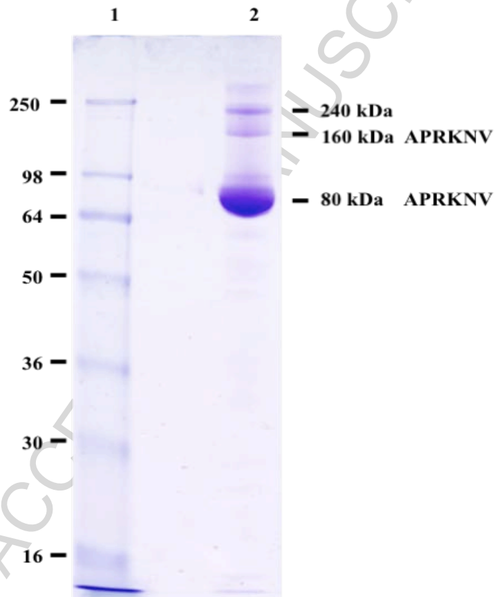
Figure 3: SDS PAGE analysis of LF. Proteins were separated using 12% Tris-Glycine SDS PAGE under non-reducing conditions and pH 8.3 following by staining with Coomassie blue R-250. Lane 1: Molecular weight marker; Lane 2: LF. N-terminal sequence analysis of the electroblotted bands is indicated.
