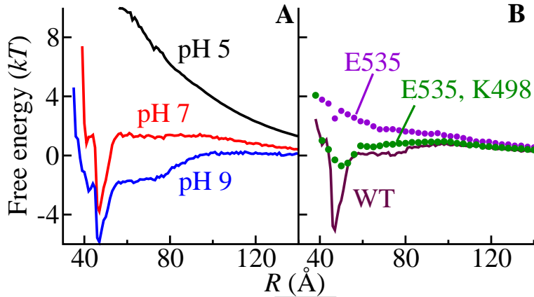
Figure 1: Free energy of interaction (PMF) between lactoferrin molecules as a function of the mass center separation, R , at (A) different pH values for the wildtype, (B) different mutations and wildtype at pH 8. The ionic strength is 5 mM in all cases. Note, one kT equals 2.48 kJ/mol at 298 K. The maximum error is about 0.2 kT .
