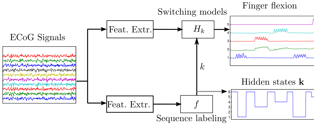
Figure 1: Diagram of the switching models decoder. We see that two models are estimated from the ECoG signals: (bottom flow) one which outputs a state k predicting which finger is moving and (top flow) another one that, given the predicted moving finger, estimates the flexion of all fingers.
