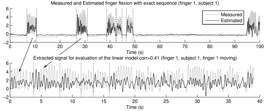
Figure 4: Signal extraction for linear model estimation: (upper plot) full signal with segmented signal, corresponding to moving finger, bracketed by the vertical lines and (lower plot) the extracted signal corresponding to the concatenation of the samples when finger 1 is moving.
