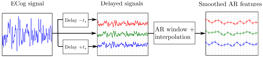
Figure 2: Diagram of the feature extraction procedure for the moving finger decoding. Here, we have outlined the processing of a single channel signal.
