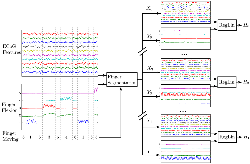
Figure 3: Workflow of the learning sets extraction ( \mathbf{X}_k and \mathbf{Y}_k ) and estimation of the coefficient matrix \mathbf{H}_k .
