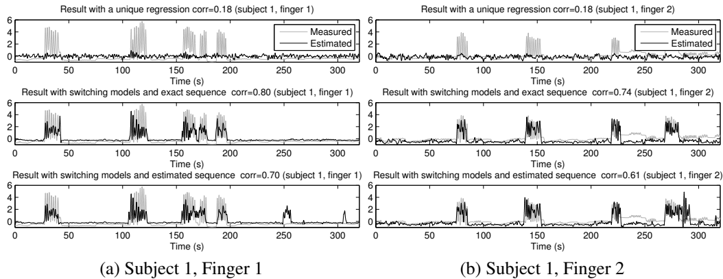
Figure 5: True and estimated finger flexion for (upper plots) a global linear regression, (middle plots) switching decoder with true moving finger segmentation and (lower plots) with the switching decoder with an estimated moving finger segmentation.
